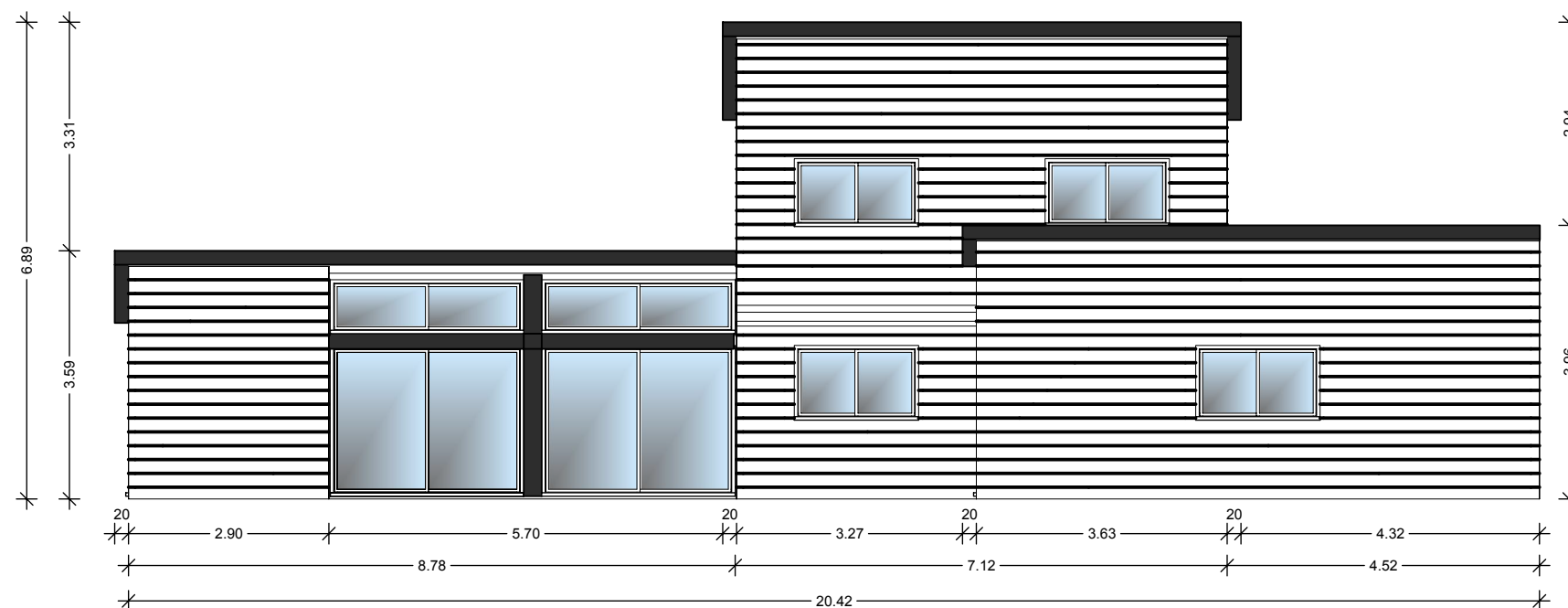
FACADE SUD
